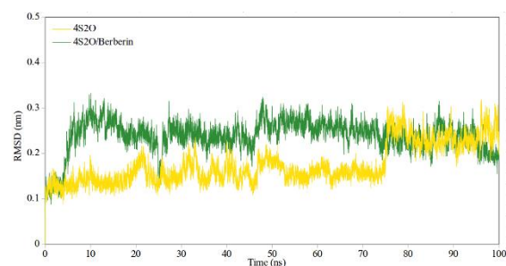
Figure 2. The time evolution of average RMSD during 100 ns MD simulations.
