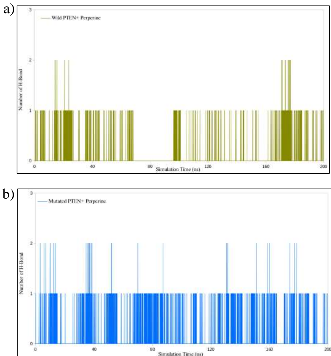
Figure 7: Time dependence of the number of hydrogen bonds between Piperine and enzymes for a) Wild-type PTEN and b) Mutated-type PTEN during the simulation time.
